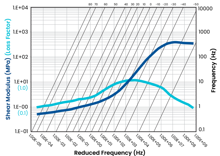
ISOLOSS™ XT-30100 Nomogram
